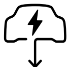
RangeXchange Icon
