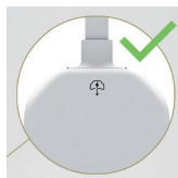
RangeXchange Icon
